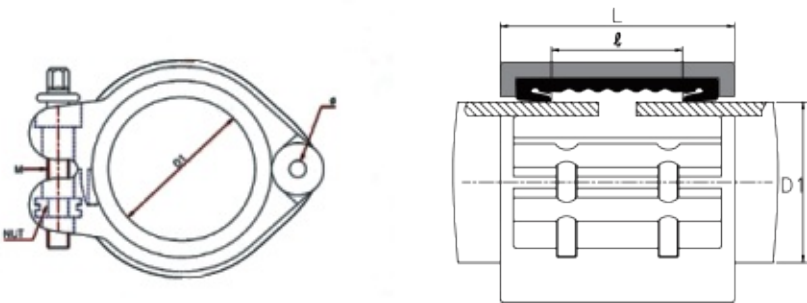
Eco-Repair Clamp Hinge Type Coupling : ERCH-S
